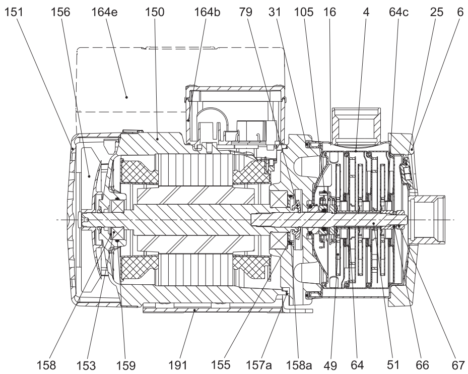
CME, CM 1-3 with MG, MGE 71 motor
