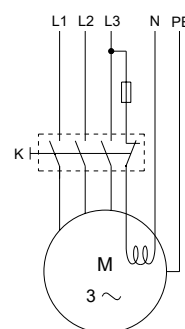
Three-phase motor with an anti-condensation heater
