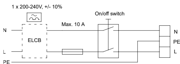
Wiring diagram, single-phase
