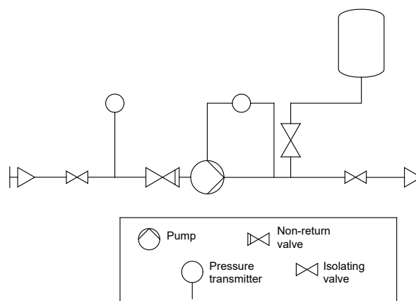
Schematic of Hydro Solo-E Optimum
