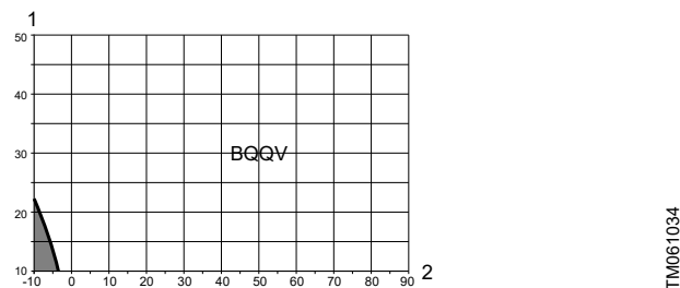
Operating range of FKM shaft seals
