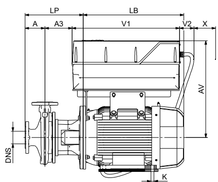
Mounting design B
