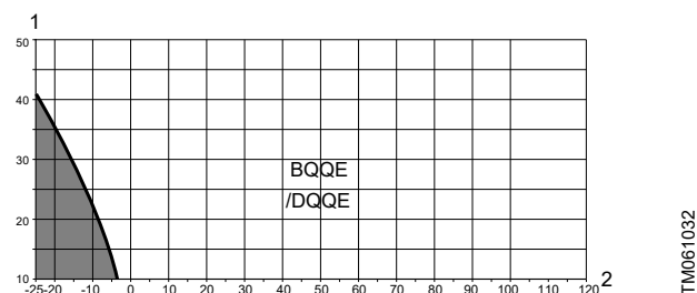
Operating range of EPDM shaft seals
