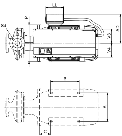
Mounting design B, with support blocks under the motor (Variant 1a in section Support blocks)
