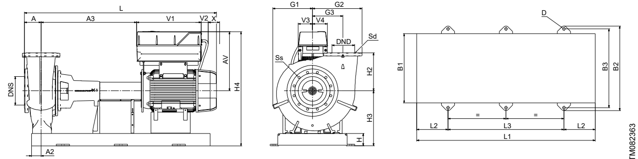
EN/ISO base frame with 6 mounting holes, tangential outlet
