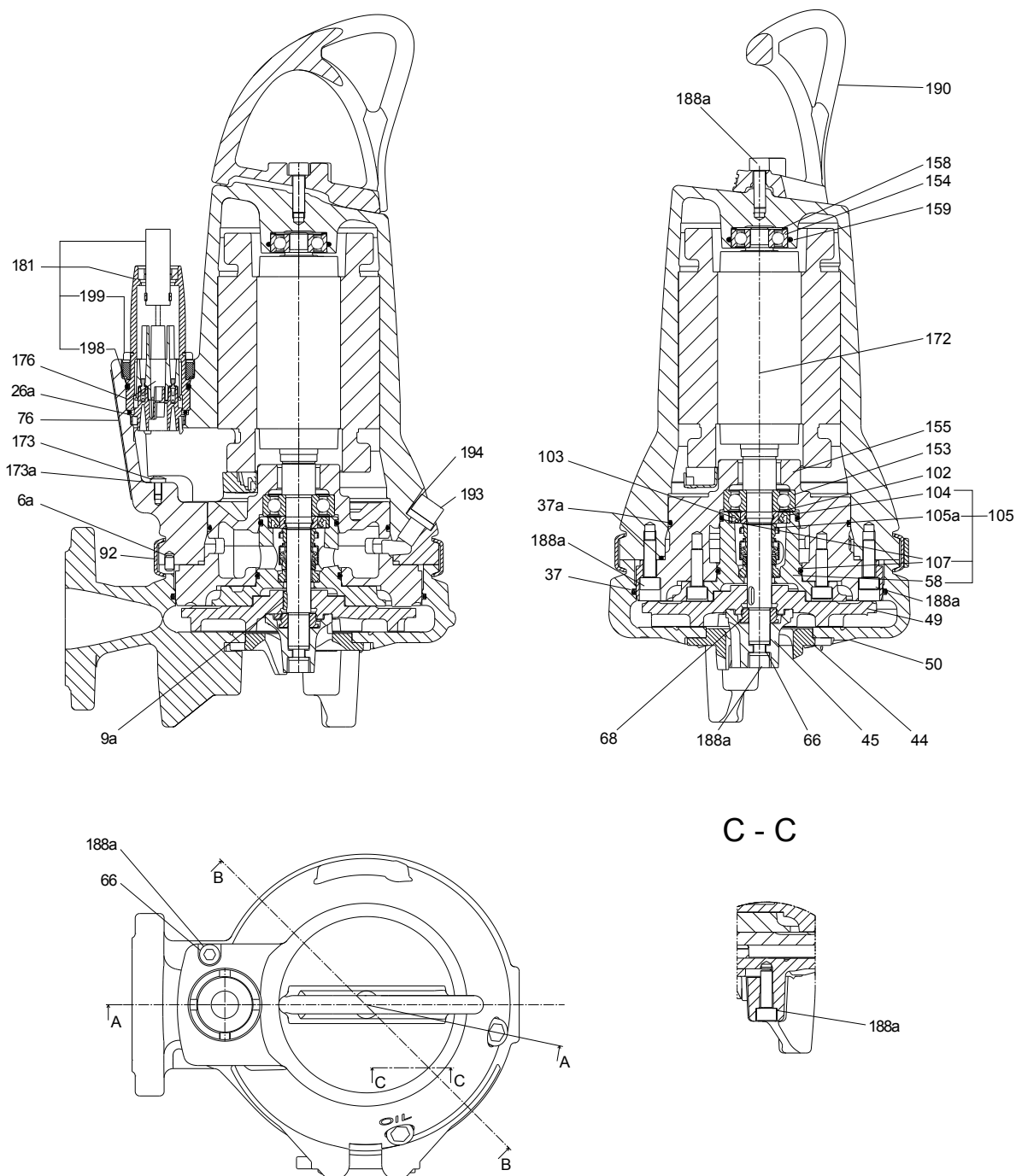
Sectional drawing of SEG pumps, 0.9, 1.2 and 1.5 kW
