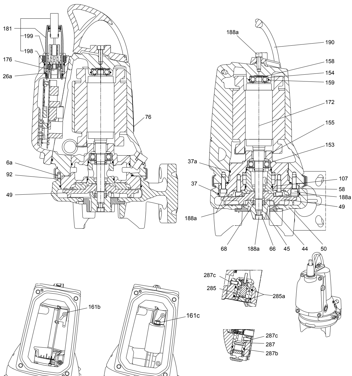
Sectional drawing of SEG AUTOADAPT pumps, 0.9, 1.2 and 1.5 kW
