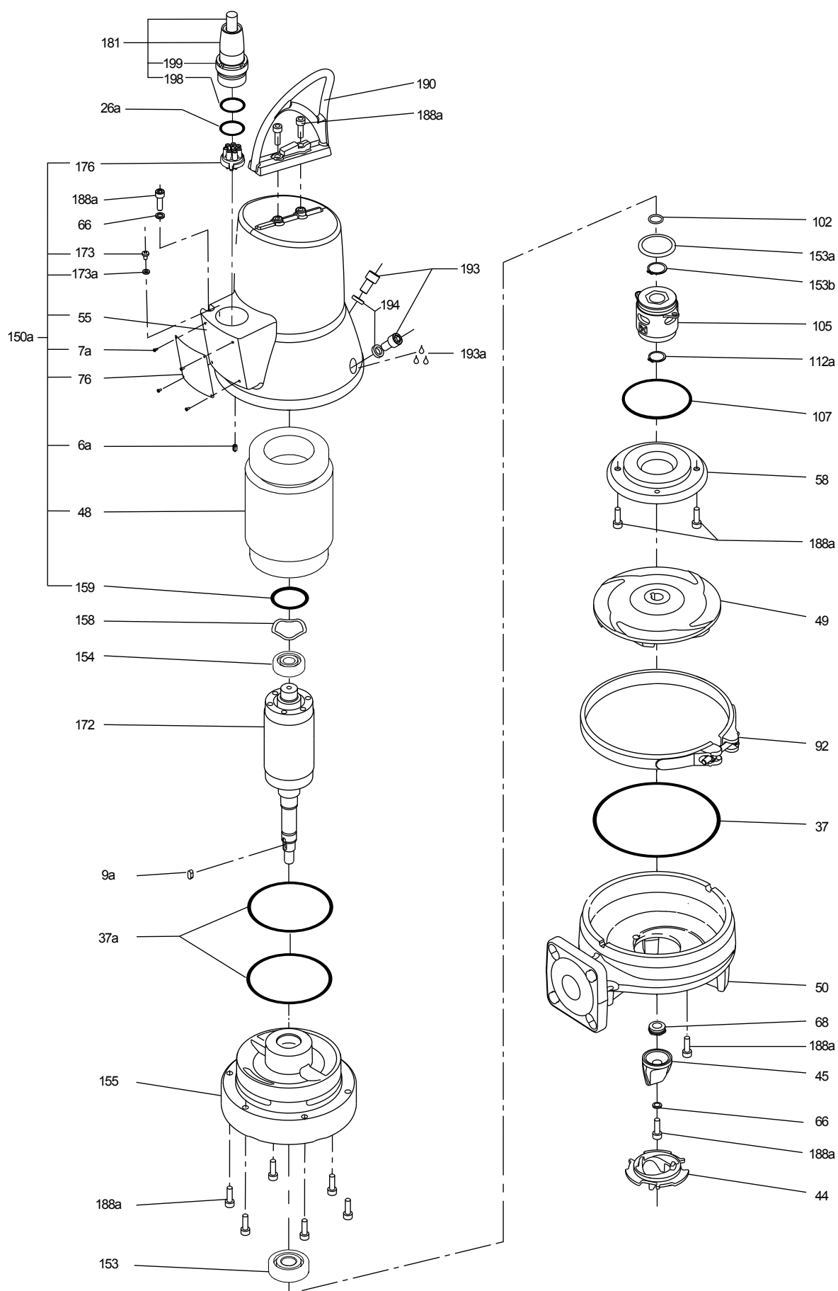
Exploded view of SEG pumps, 2.6, 3.1 and 4.0 kW
