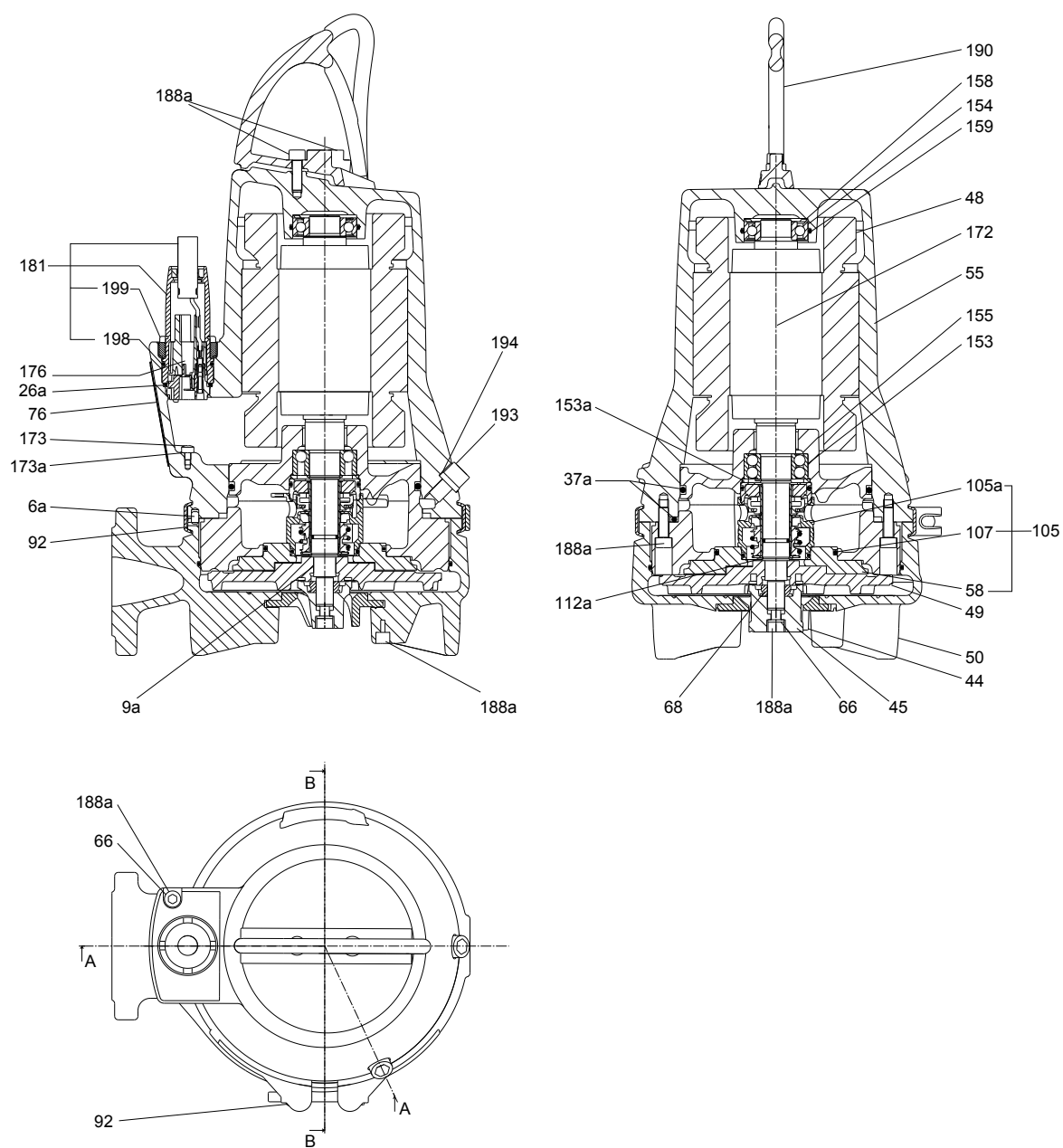
Sectional drawing of SEG pumps, 2.6, 3.1 and 4.0 kW
