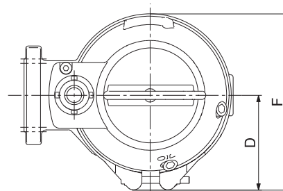
Free-standing installation with foot extensions
