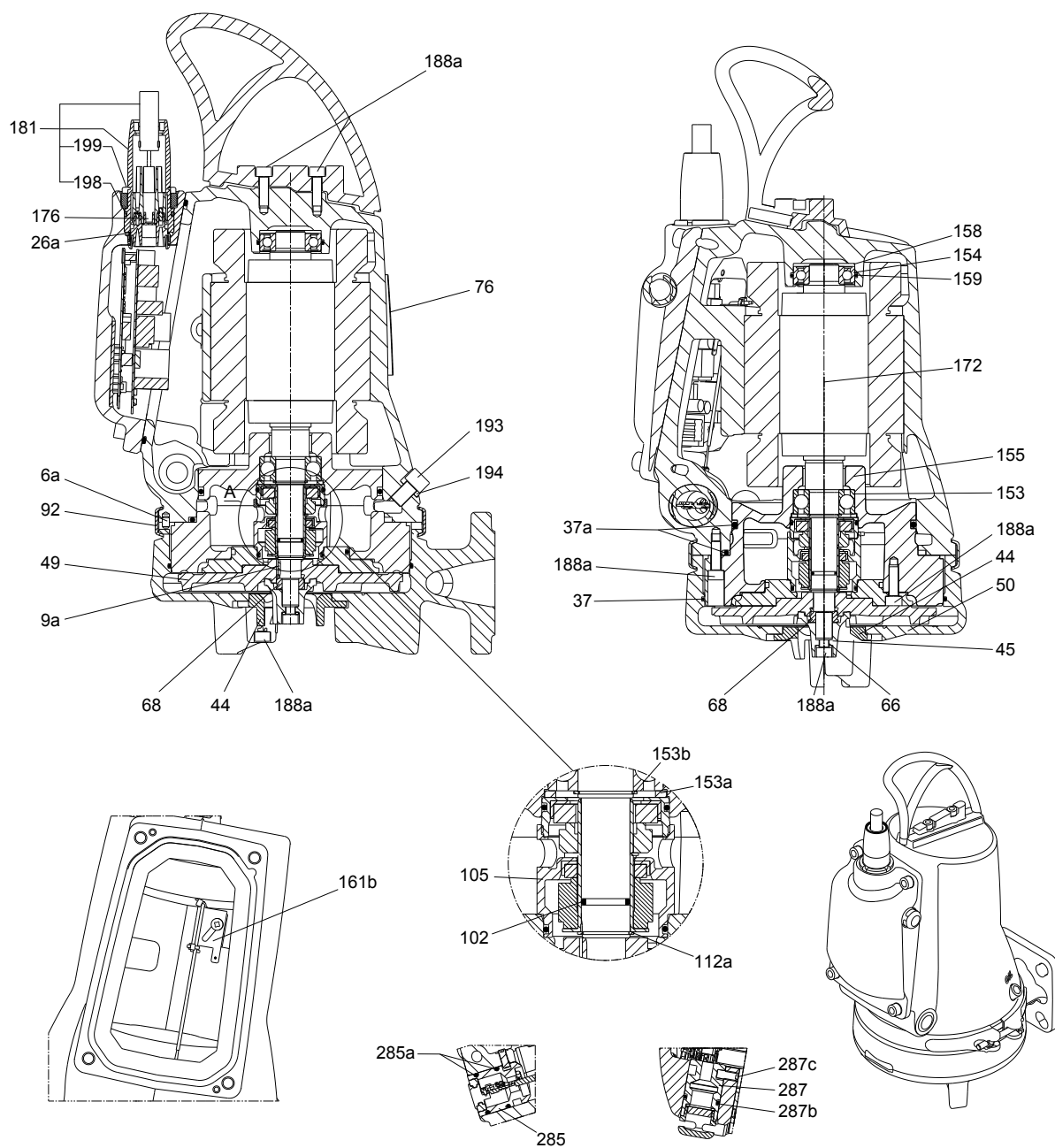
Sectional drawing of SEG AUTOADAPT pumps, 2.6, 3.1 and 4.0 kW
