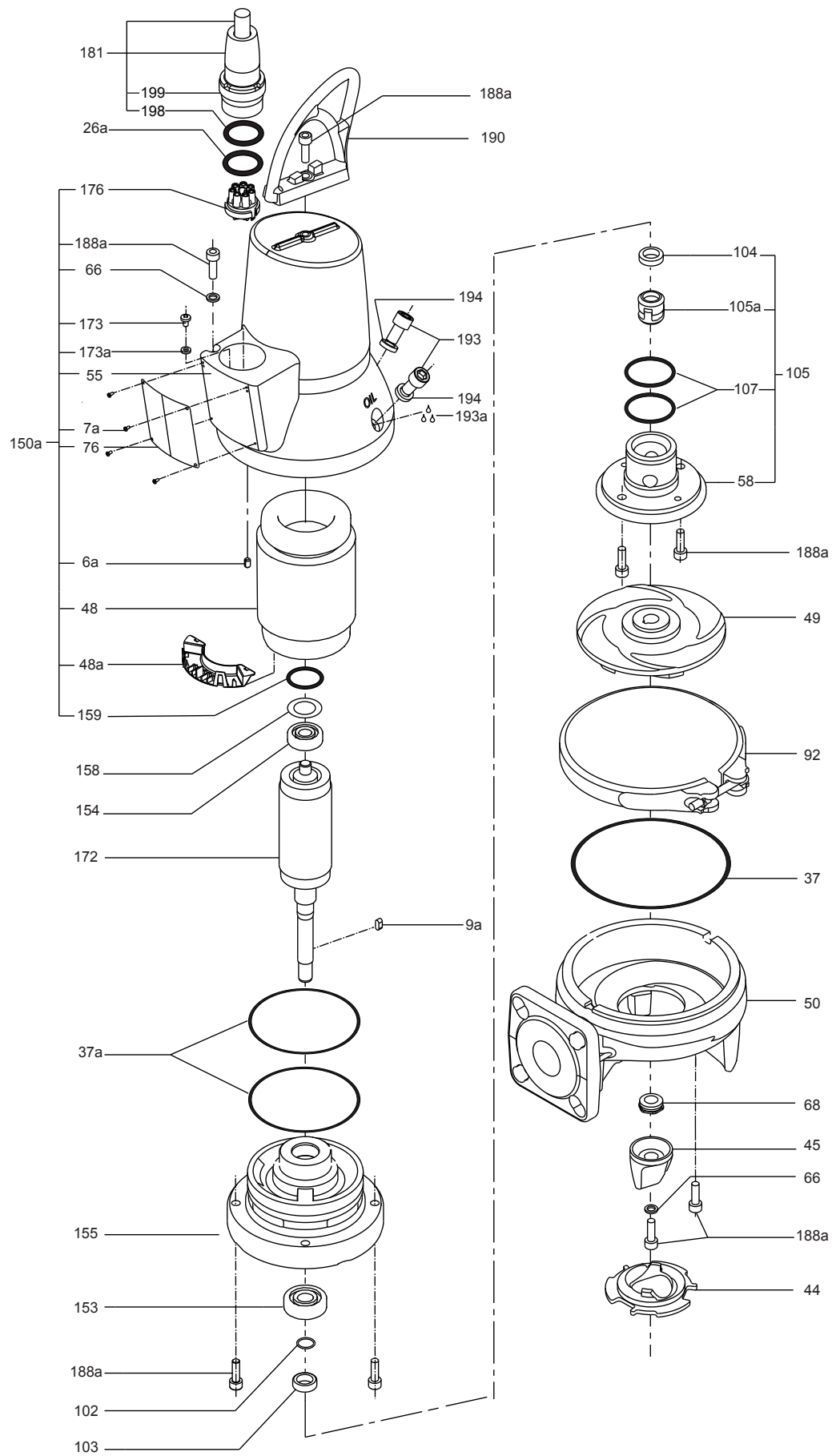
Exploded view of SEG pumps, 0.9, 1.2 and 1.5 kW
