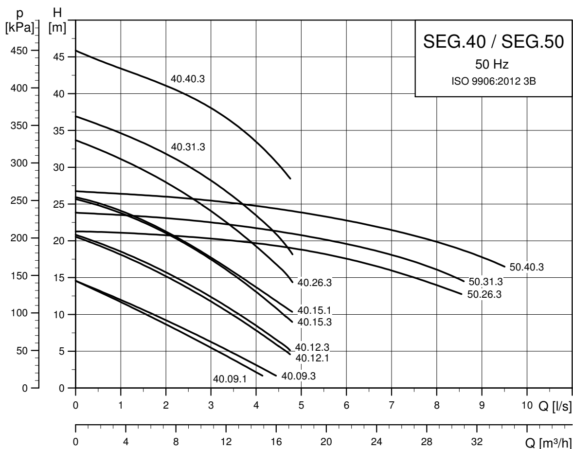
Performance range
