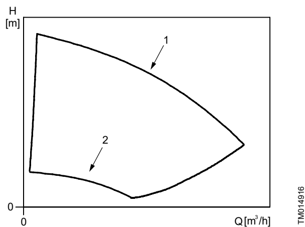
Duty range of TPE2
