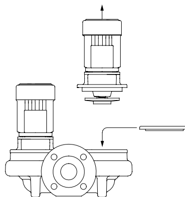
Blanking flange
