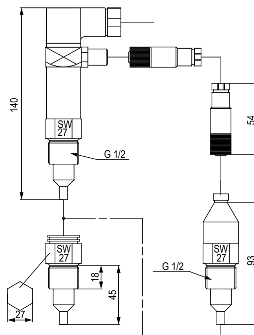
Dimensional sketch
