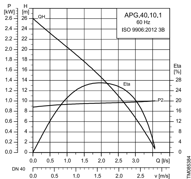
UNILIFT APG, single-phase motor
