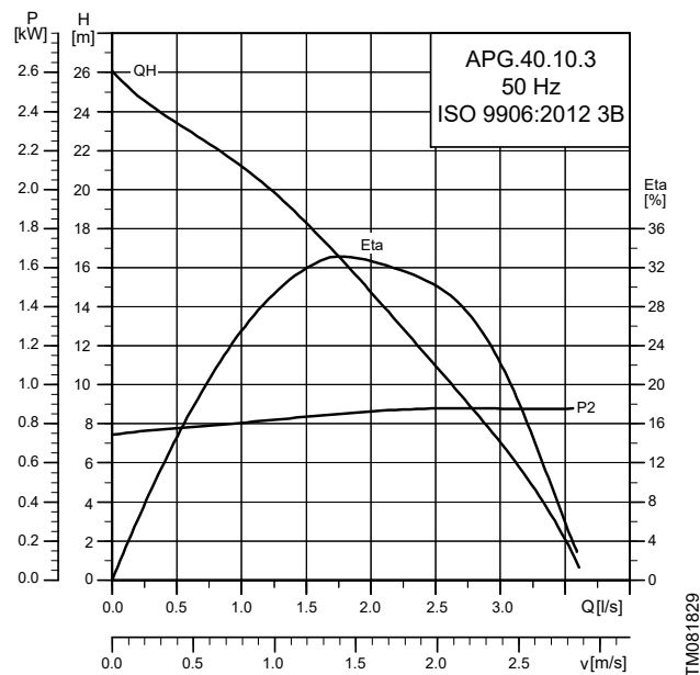
UNILIFT APG, three-phase motor
