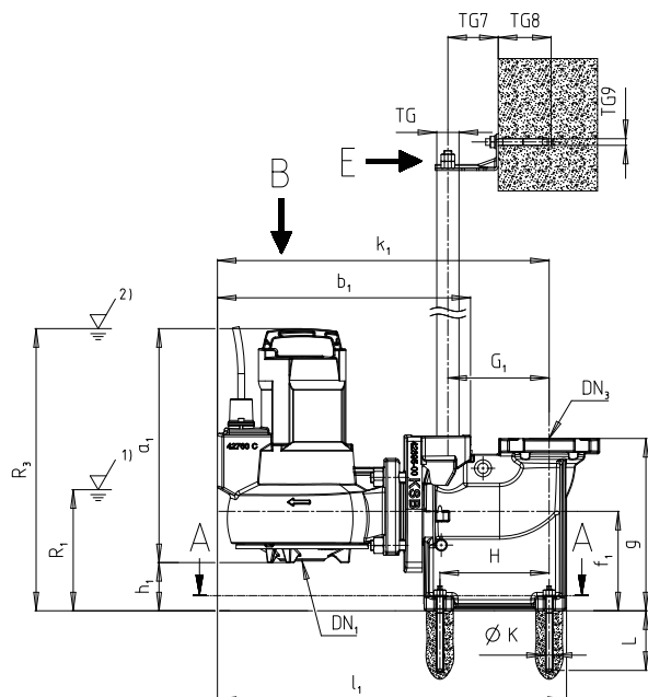
Fig. 16: Pump set dimensions, guide wire arrangement
