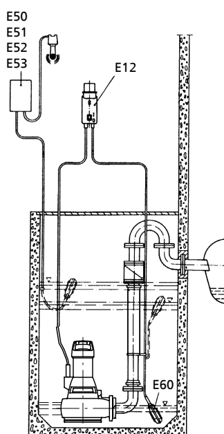
Suggested installation layout 1
