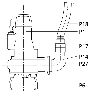
Suggested installation layout 2 Vertical hose connection with plastic hose (P18)
