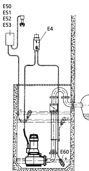
Suggested installation layout 1
