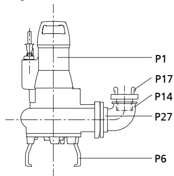
Suggested installation layout 1 Vertical hose connection with elbow (P14) and Storz rigid coupling (P17) (quick-action coupling)
