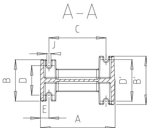
Fig. 12: Flanged bend dimensions
