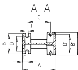
Fig. 21: Flanged bend dimensions, twin guide rail arrangement, inclined claw
