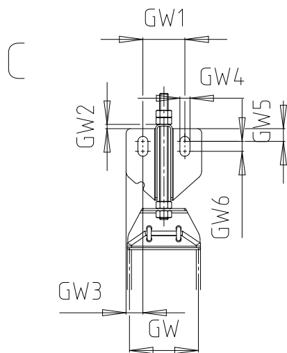
Fig. 13: Dimensions of guide wire arrangement
