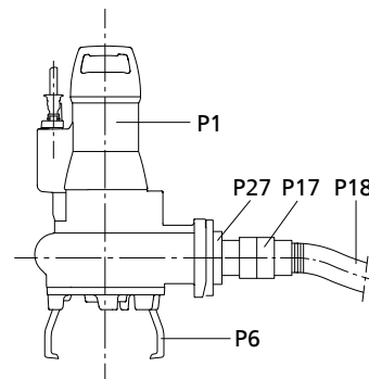
Suggested installation layout 3 Horizontal hose connection (quick-action coupling) with plastic hose (P18)
