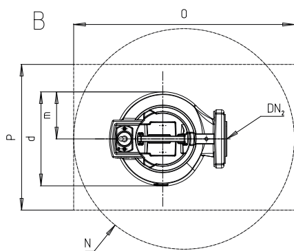
Fig. 19: Pump set dimensions, guide wire arrangement
