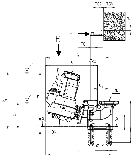
Fig. 20: AmaPorter F / S, stationary installation, twin guide rail arrangement, inclined claw
