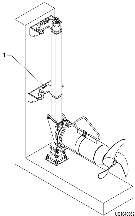
Amamix 400, 600 with guide rail 100 x 100 x 5 mm
