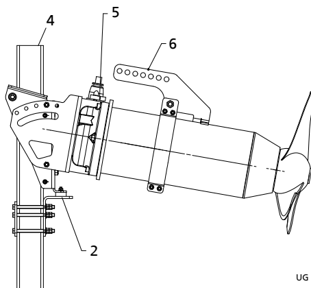
Fig. 16: Side view/isometric view
