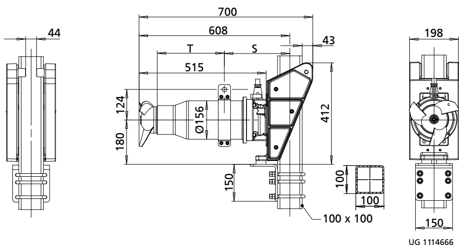
Fig. 19: Amamix 200 G: S = 215 / T = 270, motor 1 4 = 43 kg, motor 2 4 = 43.5 kg
