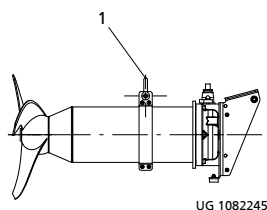
Fig. 2: Lifting tackle
