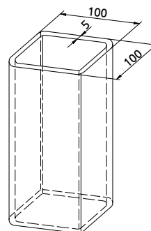
Guide rail 100 x 100 x 5 mm
