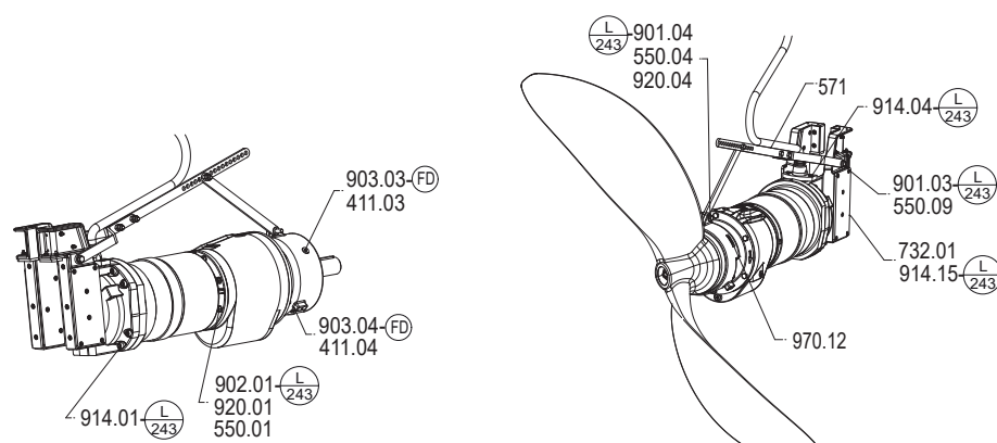
Fig. 33: External view
