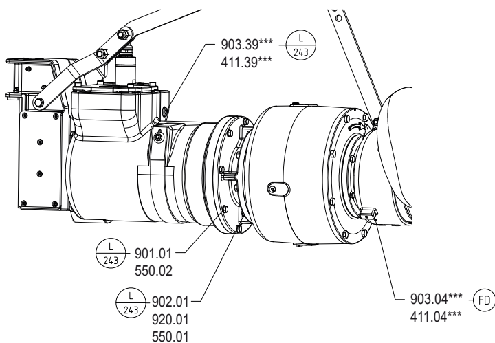
Fig. 36: External view 2
