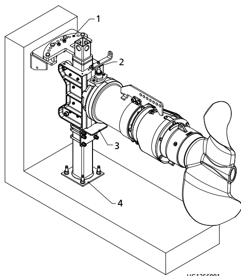
Fig. 27: Installation example: AmaProp mounted on tank wall and horizontal tank floor
