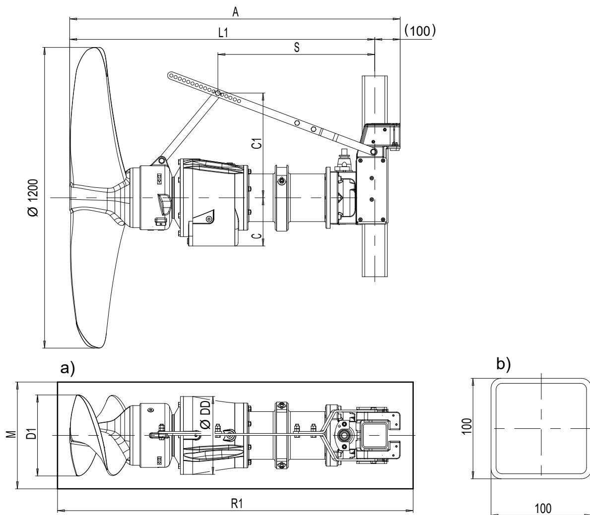
Fig. 14: AmaProp, size 1202 with three-phase asynchronous motor, dimensions in [mm]
