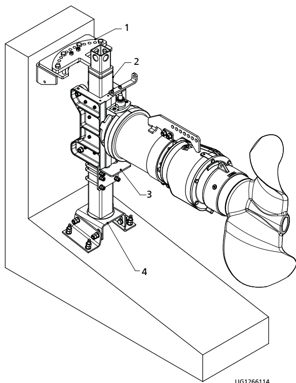
Fig. 28: Installation example: AmaProp mounted on sloping tank floor
