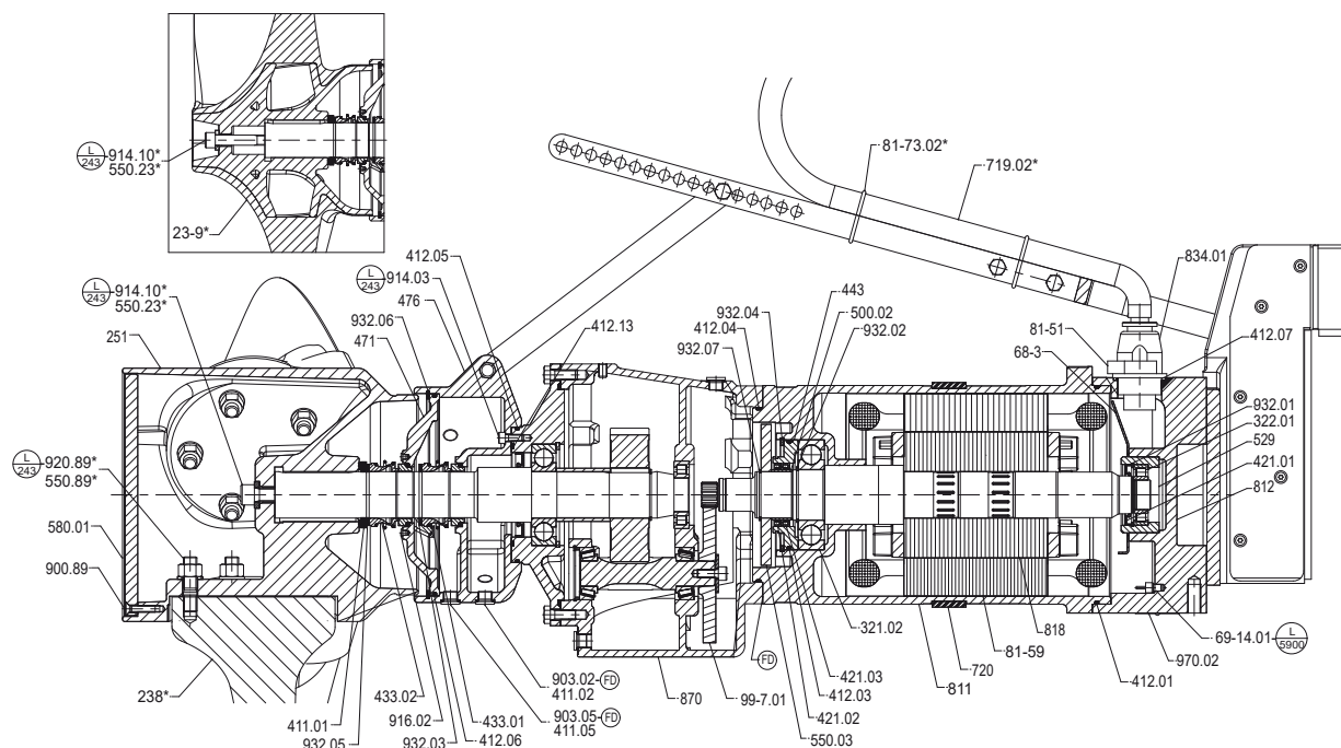
Fig. 32: General assembly drawing AmaProp, sizes 1202, 1402, 1403, 1802, 2202, 2203, 2602, 2603 with three-phase asynchronous motor
