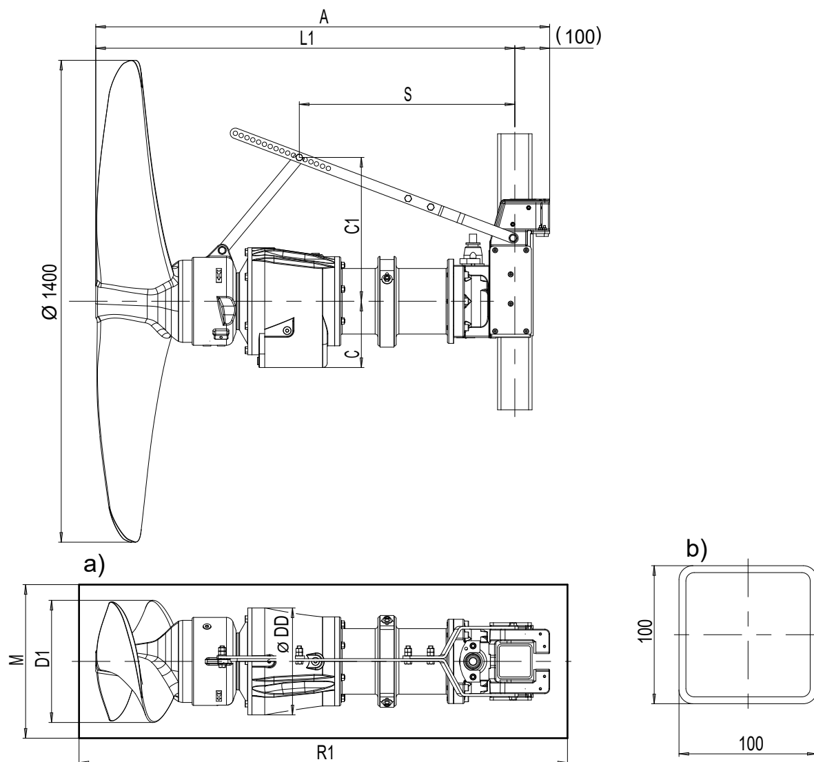
Fig. 15: AmaProp, size 1402 with three-phase asynchronous motor, dimensions in [mm]
