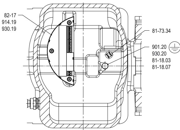
Fig. 37: Electrical connection 1
