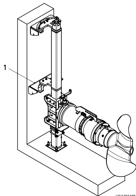
Fig. 29: Installation example: AmaProp, size 1002, mounted on tank edge and horizontal tank floor
