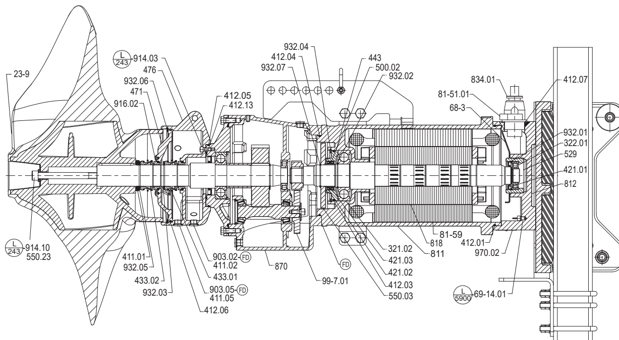
Fig. 30: General assembly drawing AmaProp, sizes 0802, 1002 with three-phase asynchronous motor
