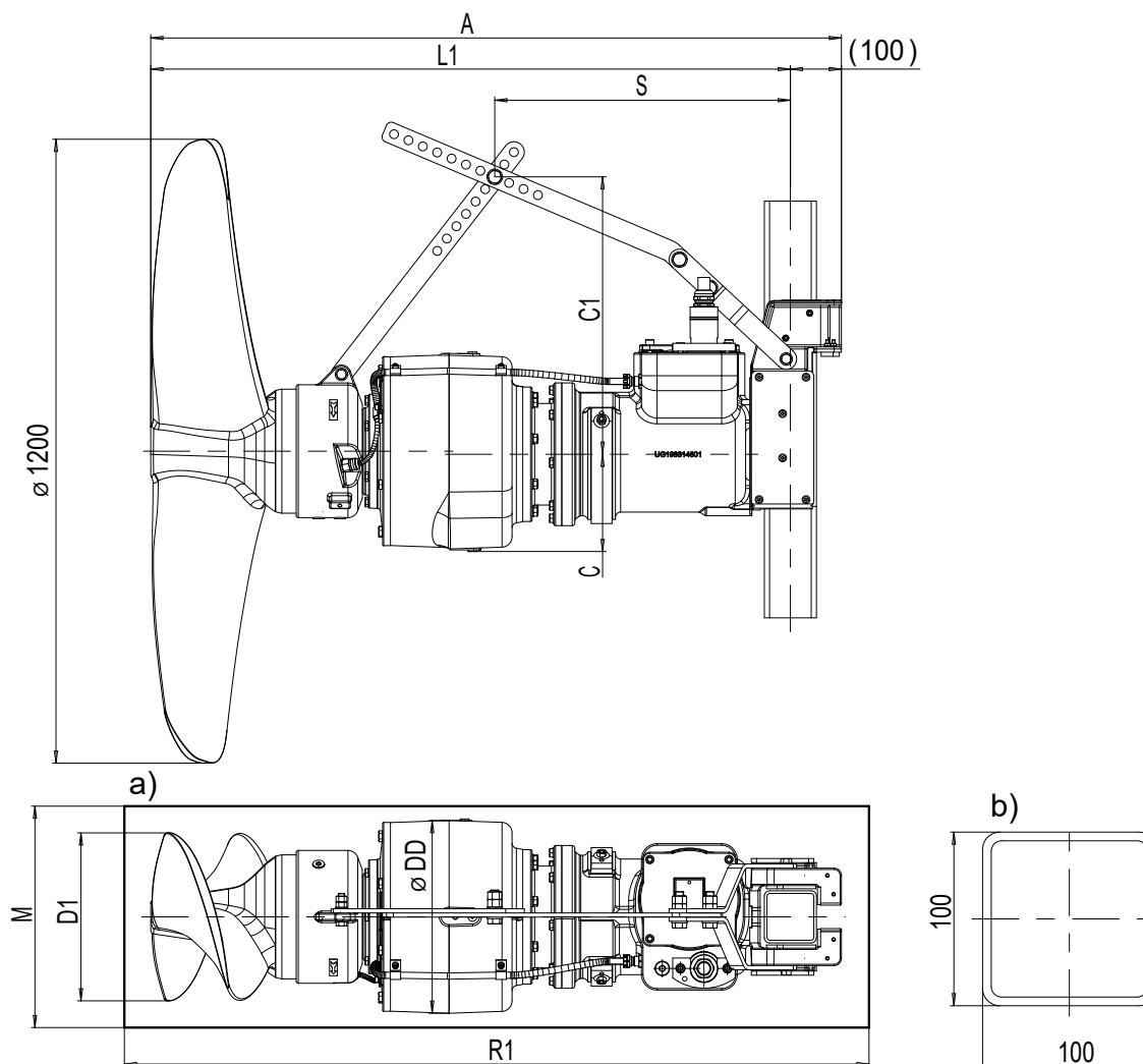
Fig. 4: AmaProp, size 1202 with synchronous reluctance motor, dimensions in [mm]
