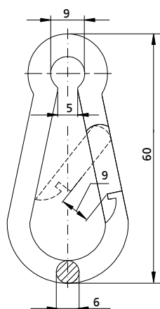
Fig. 22: Carabine hook dimensions [mm]
