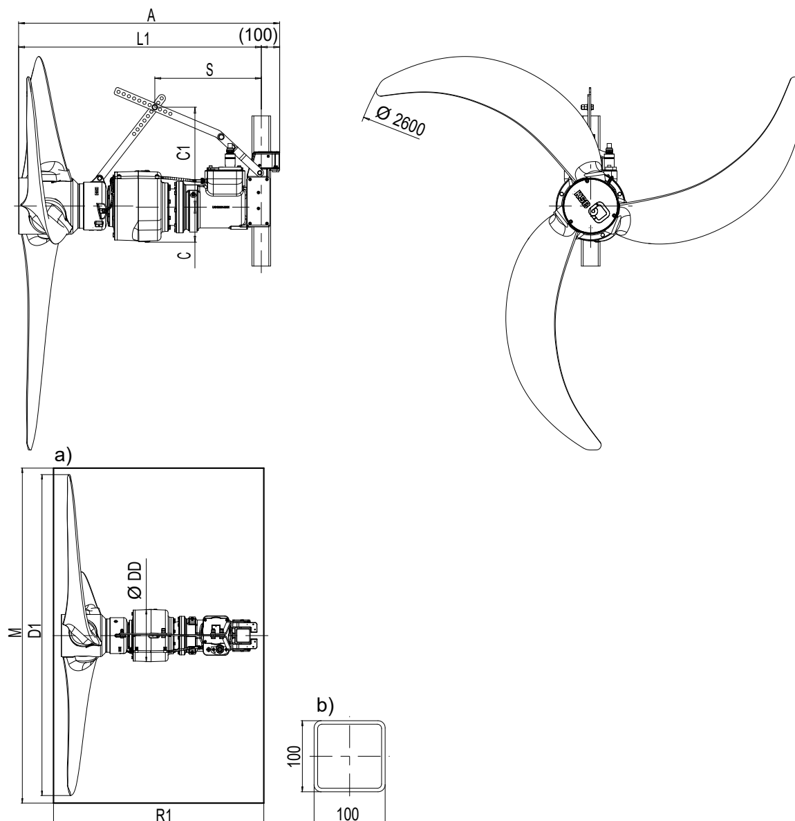
Fig. 11: AmaProp, size 2603 with synchronous reluctance motor, dimensions in [mm]
