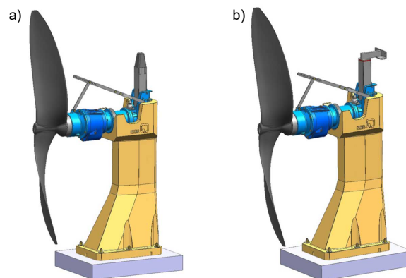
Fig. 26: Installation types
