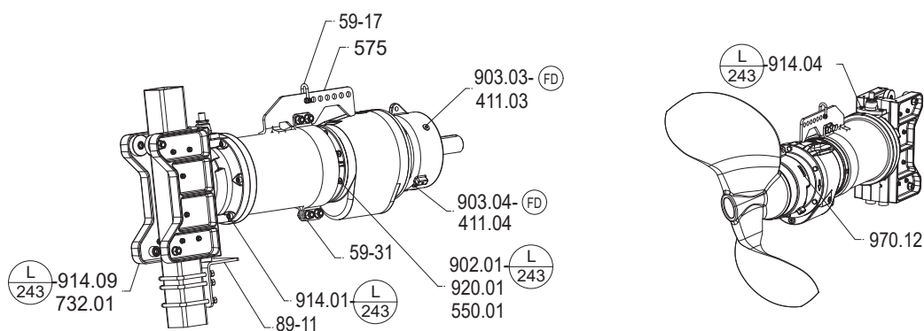
Fig. 31: External view
