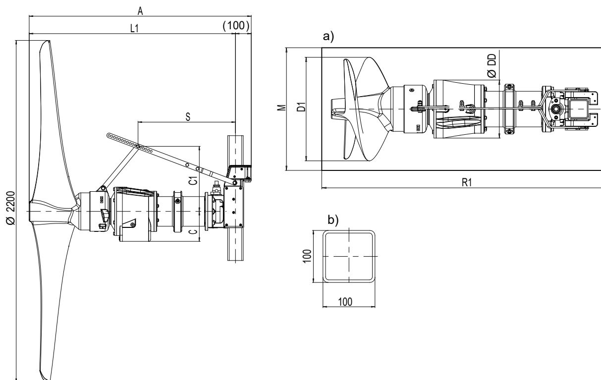
Fig. 17: AmaProp, size 2202 with three-phase asynchronous motor, dimensions in [mm]
