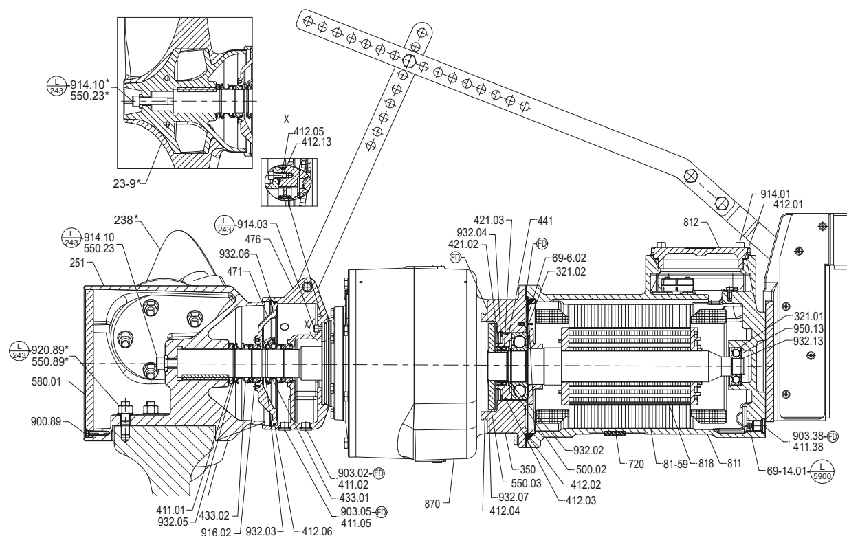
Fig. 34: General assembly drawing AmaProp with synchronous reluctance motor * To be assembled on site
