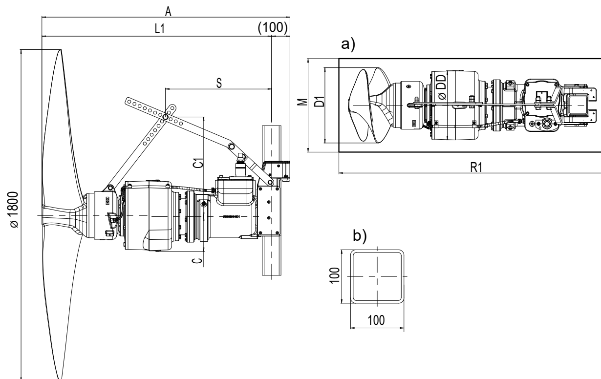
Fig. 6: AmaProp, size 1802 with synchronous reluctance motor, dimensions in [mm]
