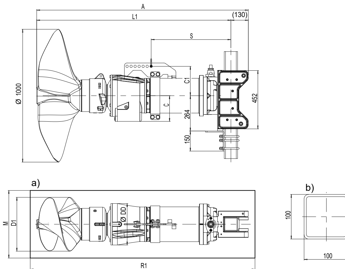
Fig. 13: AmaProp, size 1002 with three-phase asynchronous motor, dimensions in [mm]
