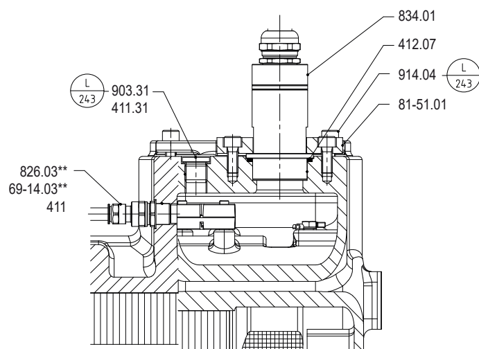
Fig. 38: Electrical connection 2
