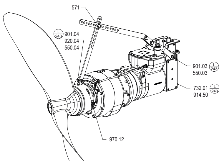
Fig. 35: External view 1
