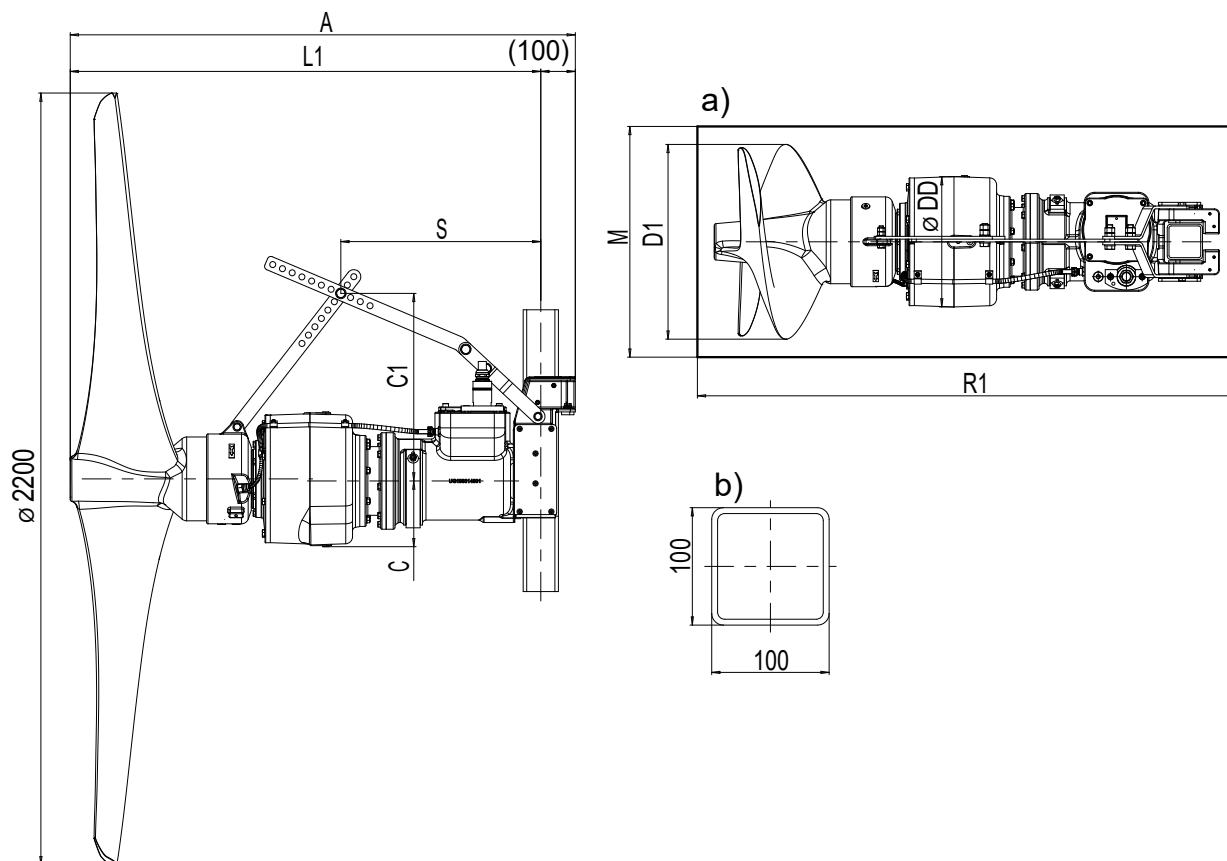
Fig. 7: AmaProp, size 2202 with synchronous reluctance motor, dimensions in [mm]
