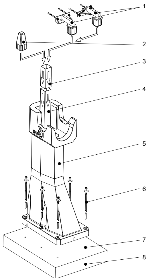
Fig. 25: General assembly drawing
