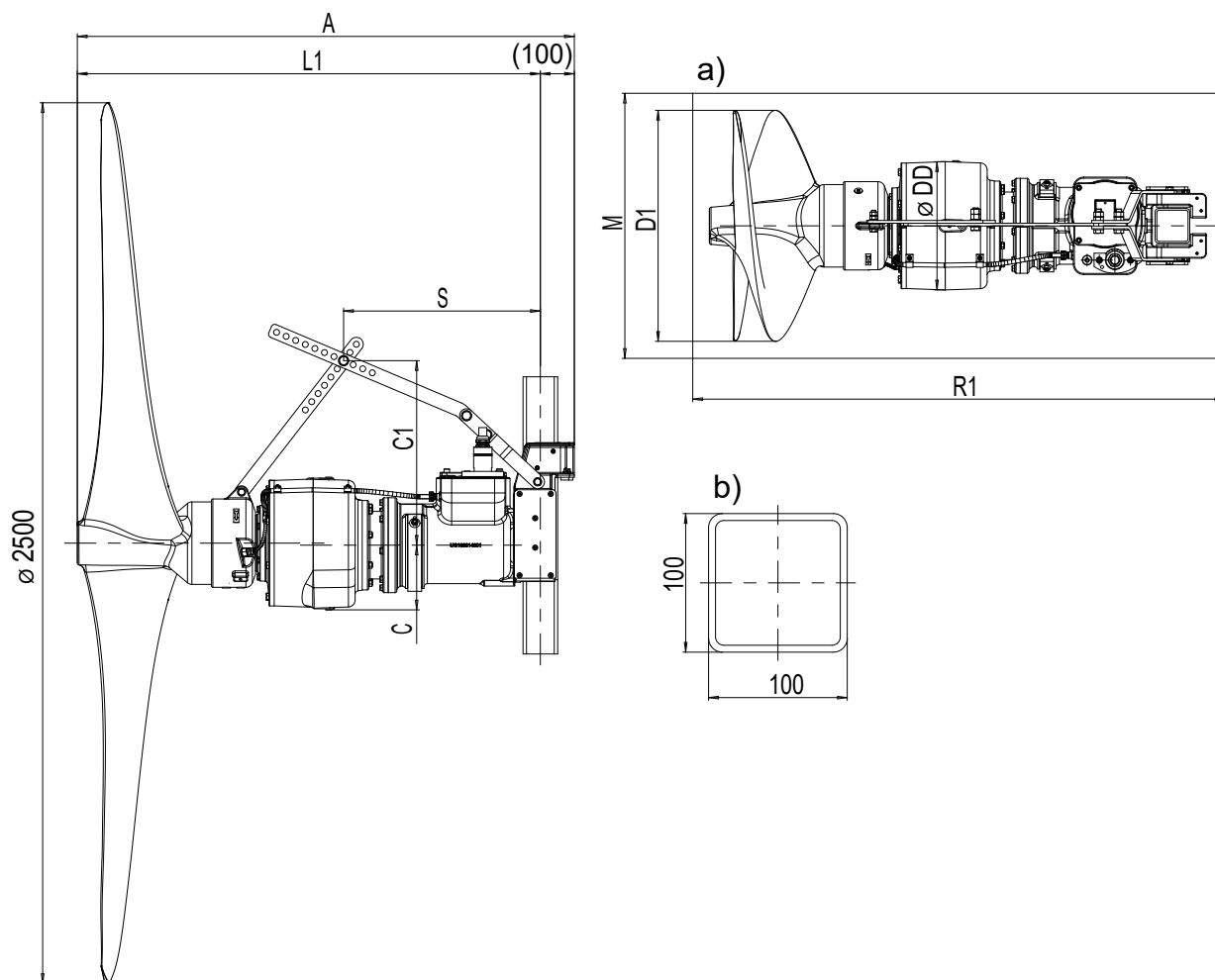
Fig. 8: AmaProp, size 2602 with synchronous reluctance motor, dimensions in [mm]
