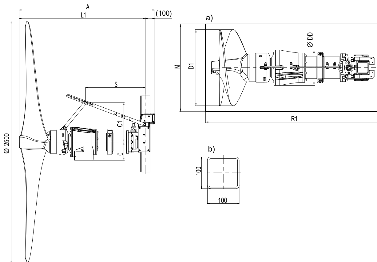
Fig. 18: AmaProp, size 2602 with three-phase asynchronous motor, dimensions in [mm]
