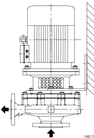
Fig. 25: Pump foot, fastened at the side, up to motor size 112 = 4 kW
