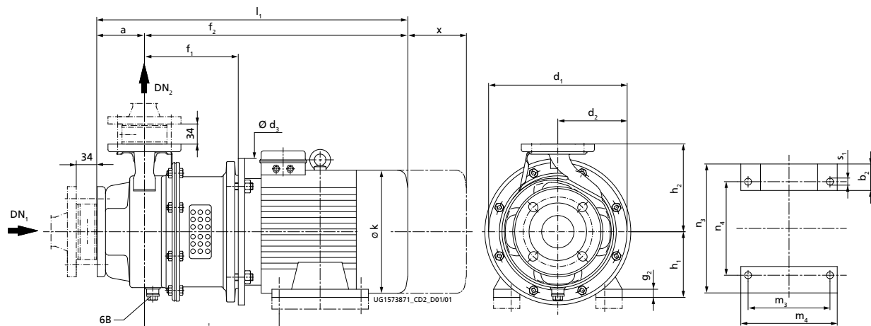
Fig. 11: Etachrom B with motor foot, dimensions [mm]
