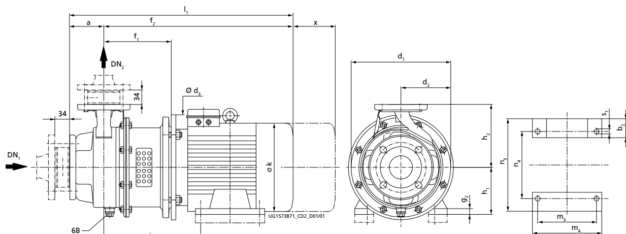
Fig. 15: Etachrom B with motor foot, dimensions [mm]
