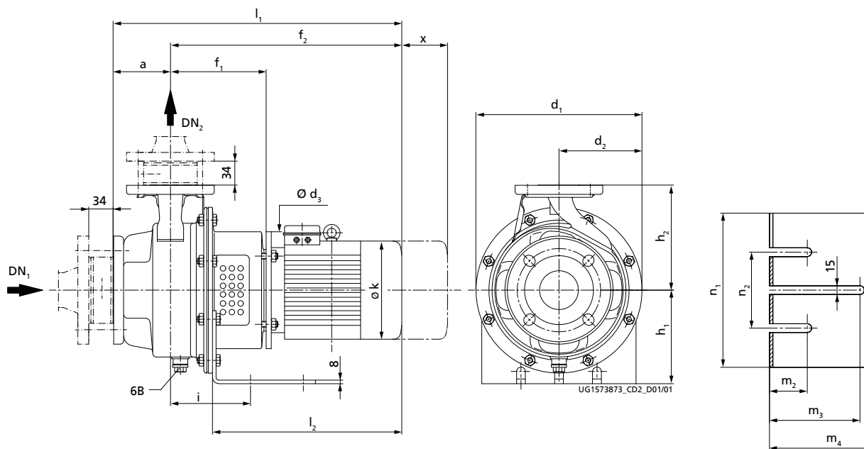
Fig. 4: Etachrom B with pump foot, dimensions [mm]
