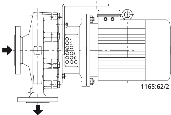
Fig. 19: Pump foot, fastened above, up to motor size 112 = 4 kW The motor must be turned by 180°.
