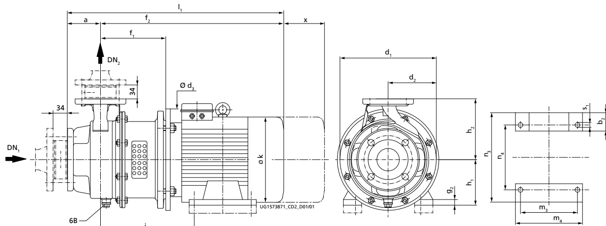
Fig. 14: Etachrom B with motor foot, dimensions [mm]
