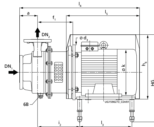
Etachrom B with 4-point ball feet, with motor shroud
