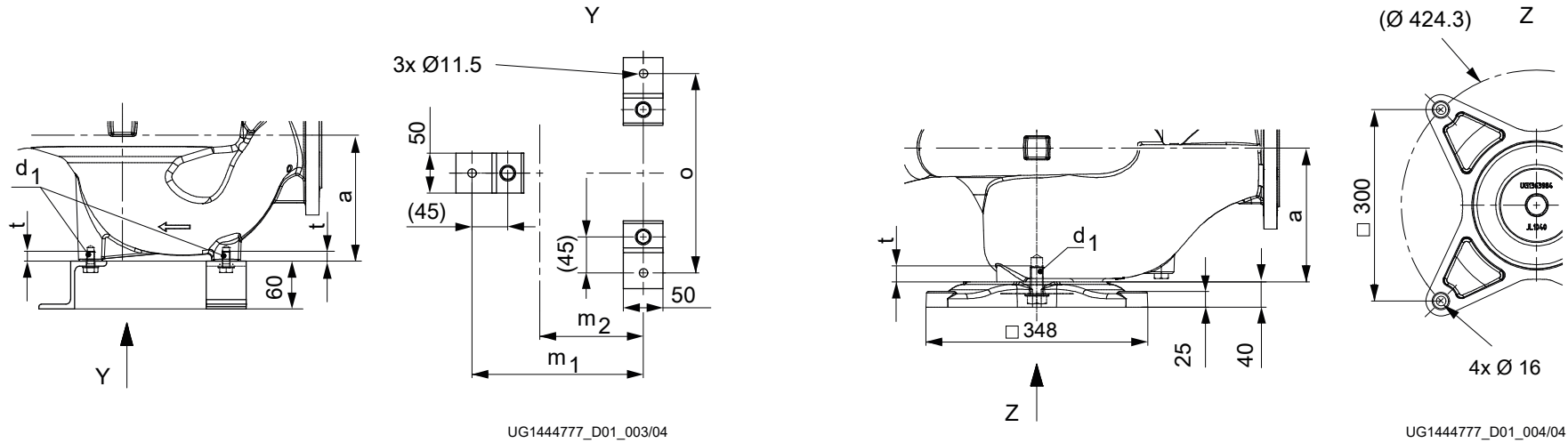
Fig. 3: Foundation fastening dimensions [mm]
