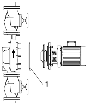
Fig. 13: Horizontal installation with blind flange (1 = blind flange, accessory)
