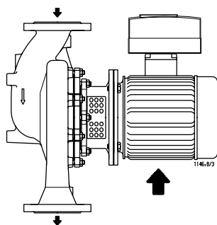
Fig. 11: Horizontal installation of pump sets with PumpDrive, direction of flow from top to bottom
