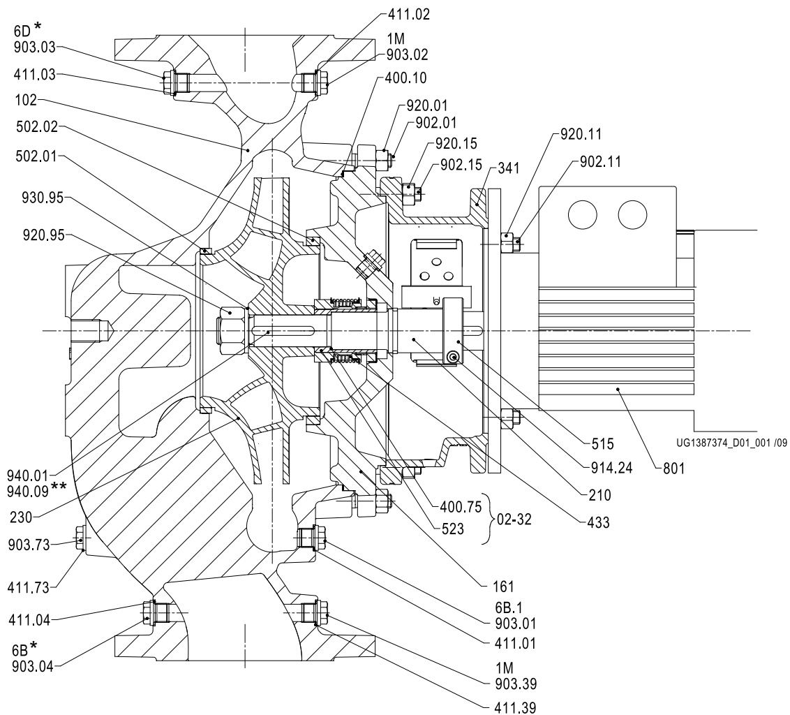
Fig. 19: General assembly drawing
