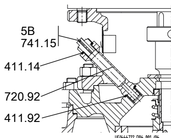
Fig. 21: Vent valve 5B for vertical installation
