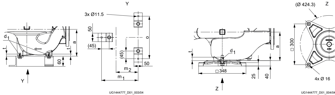
Fig. 5: Foundation fastening dimensions [mm]
