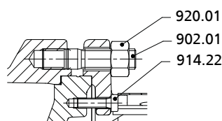
Fig. 22: Fastening elements for the clamped casing cover
