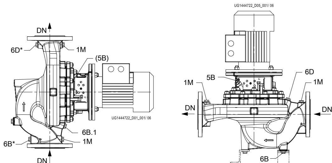
Fig. 6: Connections * = optional
