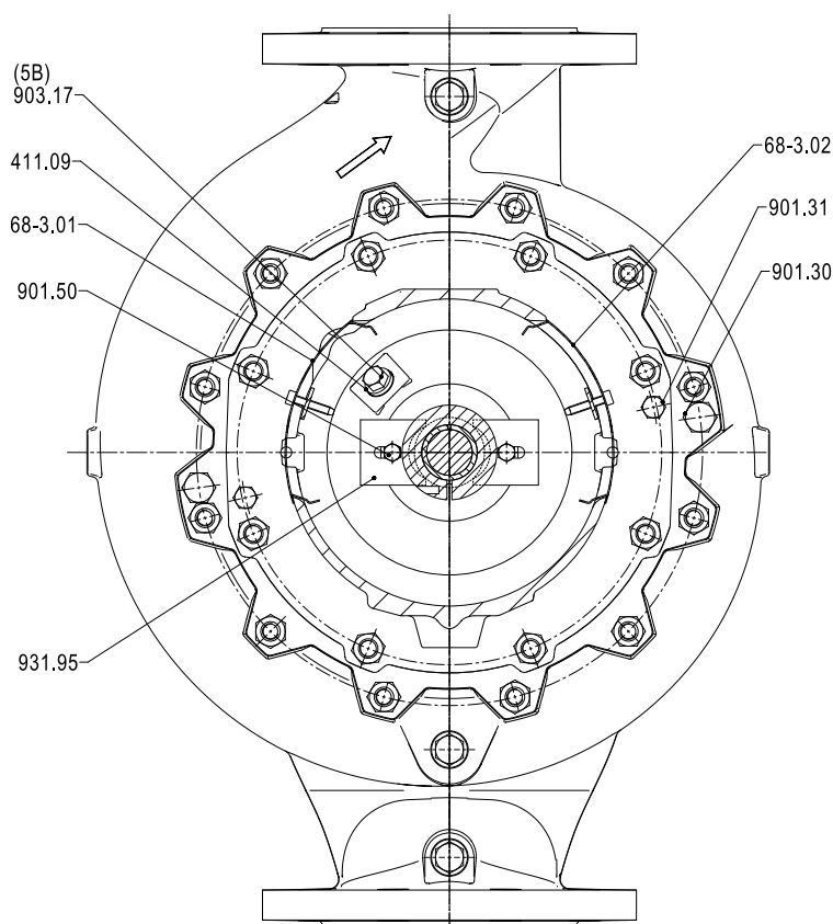
Fig. 20: General assembly drawing: side view (pump in operation)
