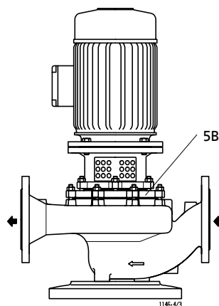
Fig. 17: Vertical installation
