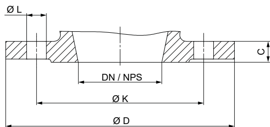
Fig. 7: Flange dimensions
