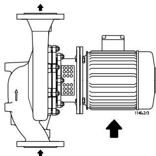
Fig. 8: Horizontal installation, direction of flow from bottom to top
