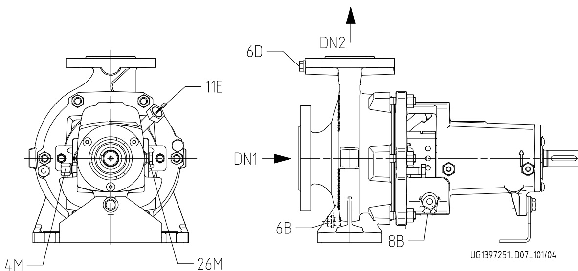
Fig. 7: Version with grease lubrication, with hole for connecting measuring equipment, no connection for pressure gauge
