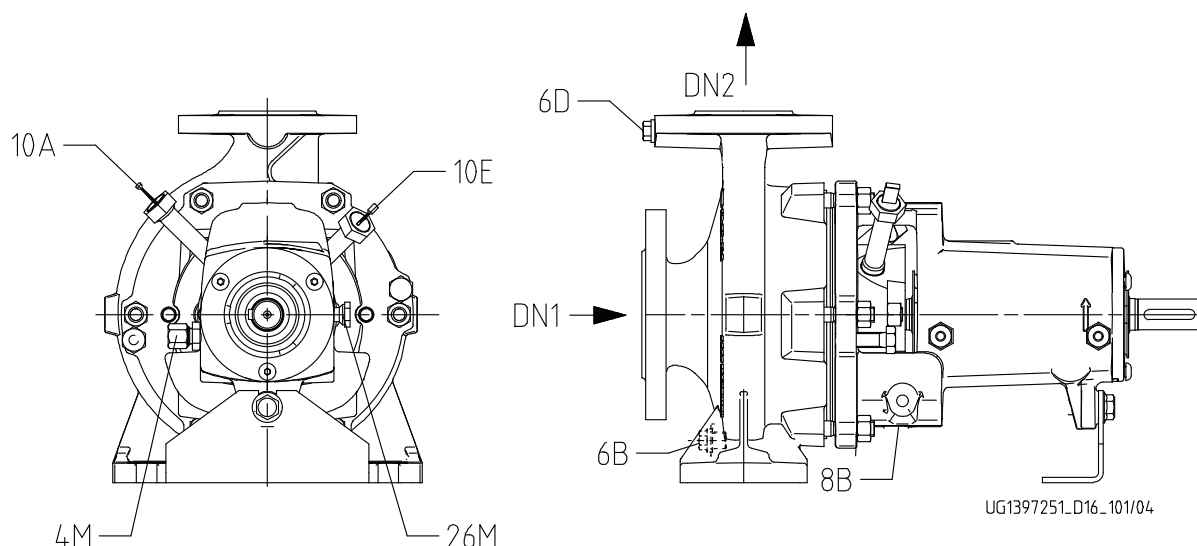
Fig. 10: Version with grease lubrication, with hole for connecting measuring equipment, no connection for pressure gauge
