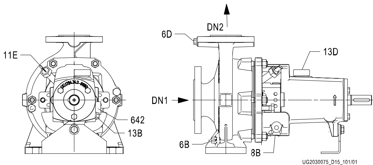
Fig. 6: Version with oil level sight glass, no hole for connecting measuring equipment, no connection for pressure gauge
