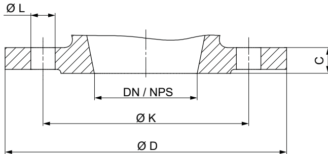
Fig. 11: Flange dimensions
