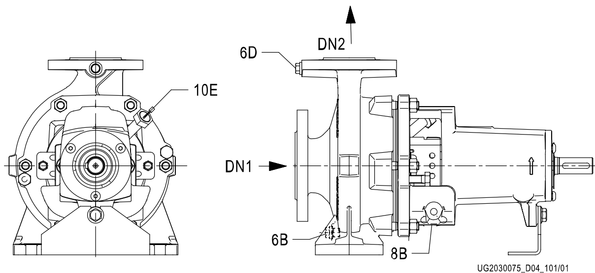
Fig. 8: Version with grease lubrication, no hole for connecting measuring equipment, no connection for pressure gauge
