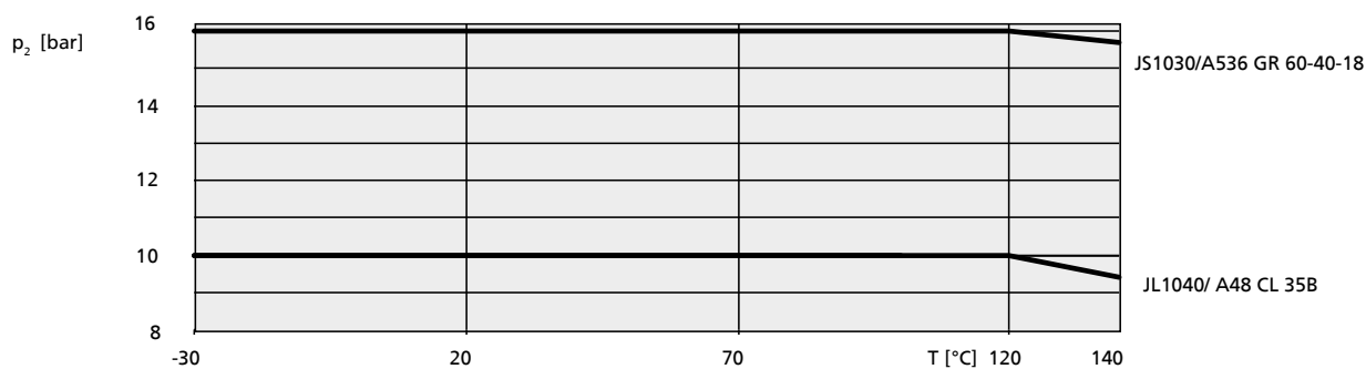
Fig. 3: Pump pressure limits and temperature limits 36) ETNE 34)
