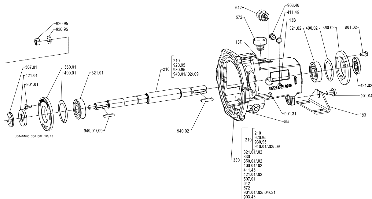
Fig. 25: Version with oil lubrication and oil level sight glass
