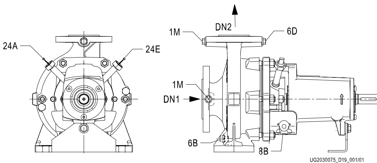
Fig. 9: Version with grease lubrication, no hole for connecting measuring equipment, with connection for pressure gauge
