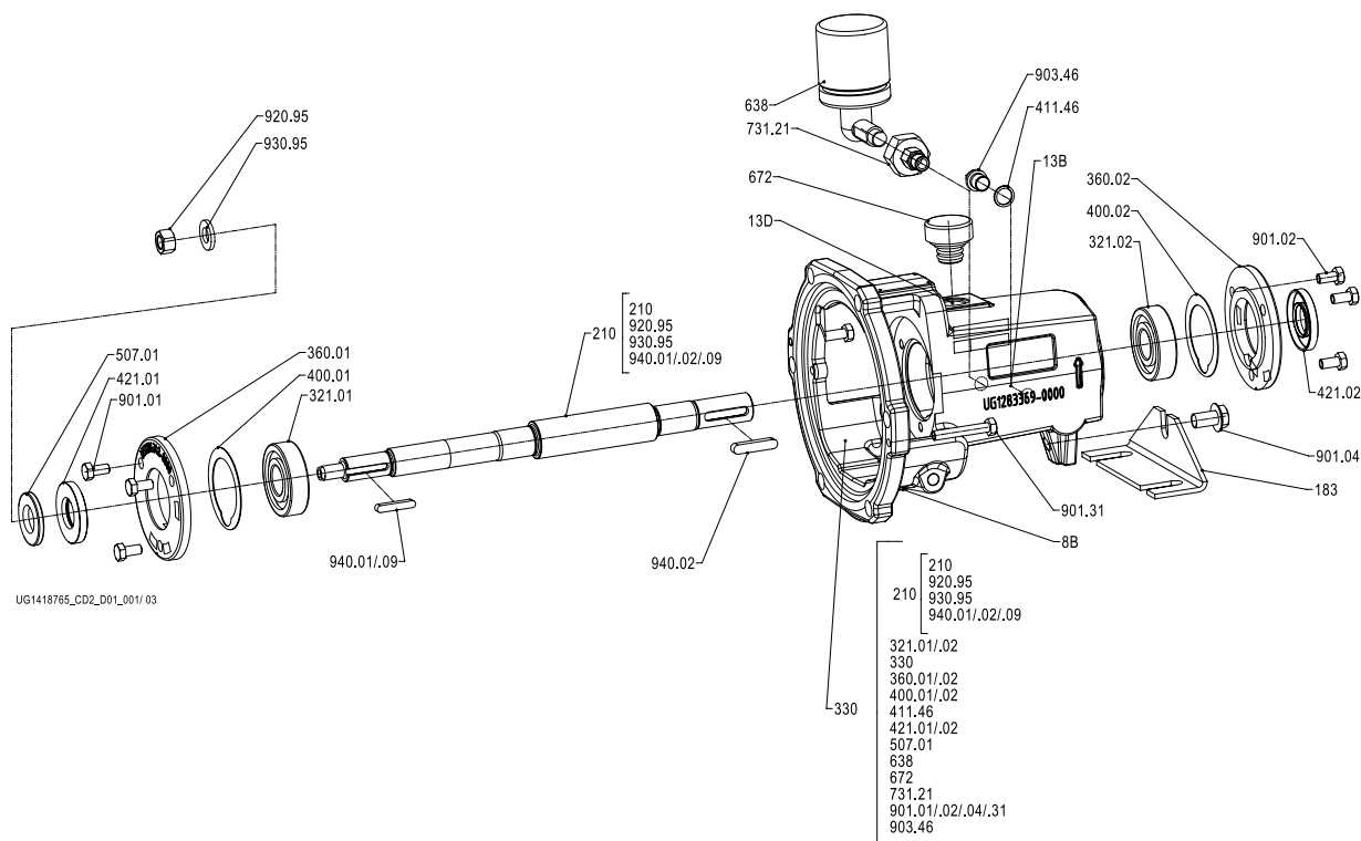
Fig. 23: Version with oil lubrication and constant level oiler
