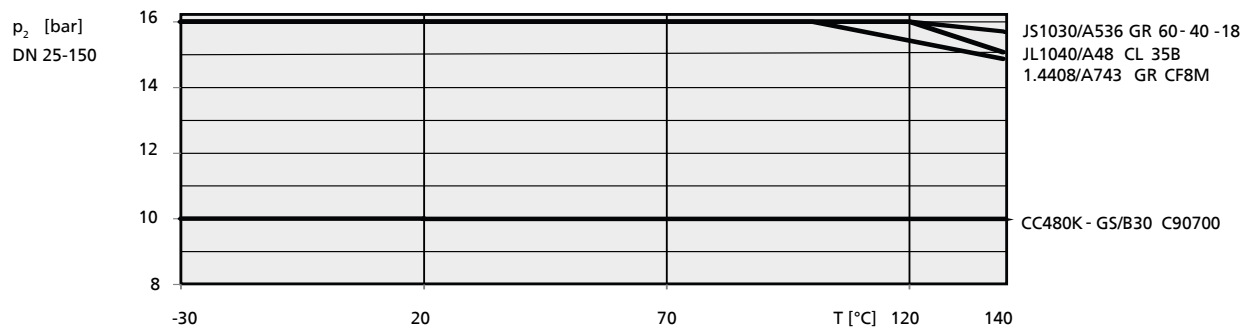
Fig. 1: Pump pressure limits and temperature limits DN 25 - DN 150 for ETN 35)
