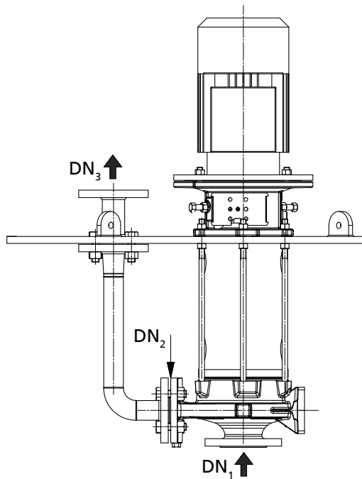
Fig. 5: Flange designation
