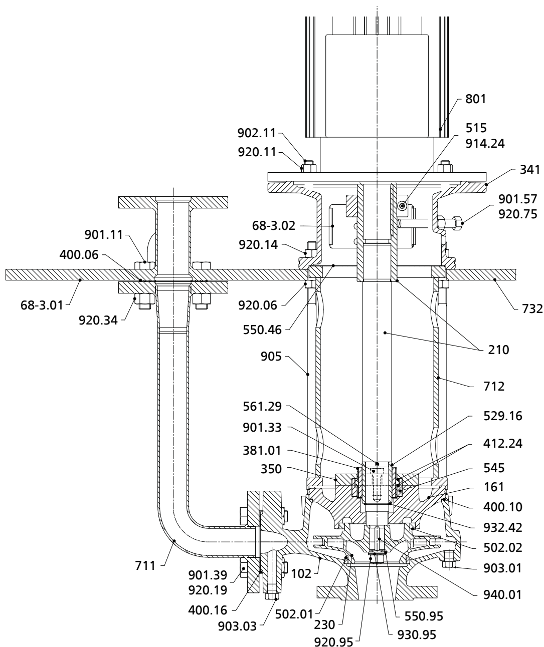
Fig. 7: General assembly drawing of Etanorm V, design W
