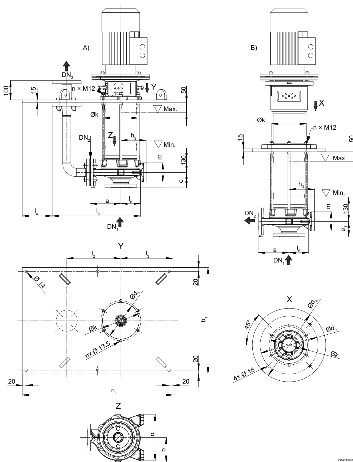
Fig. 1: Dimensions [mm]
