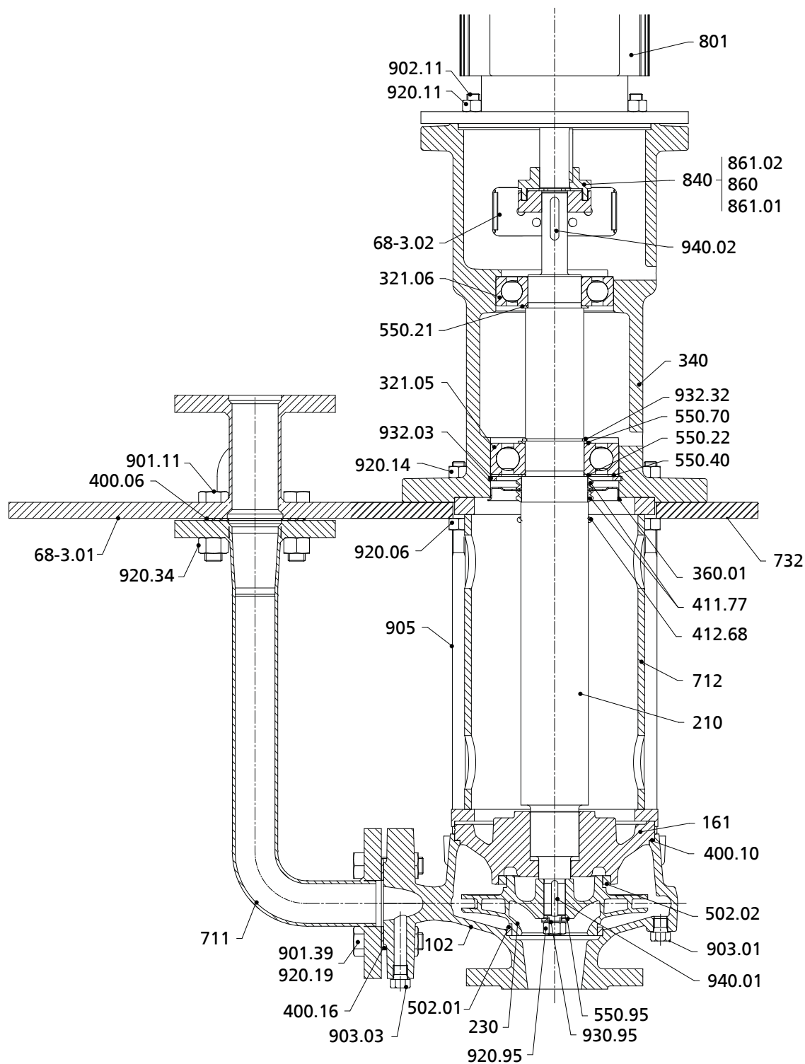
Fig. 6: General assembly drawing of Etanorm V, design D
