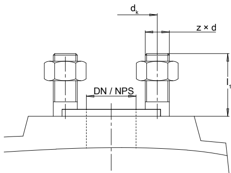
Fig. 5: Flange dimensions
