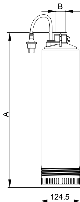
Fig. 1: Pump set dimensions
