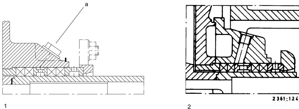
Fig. 1: Gland packing
