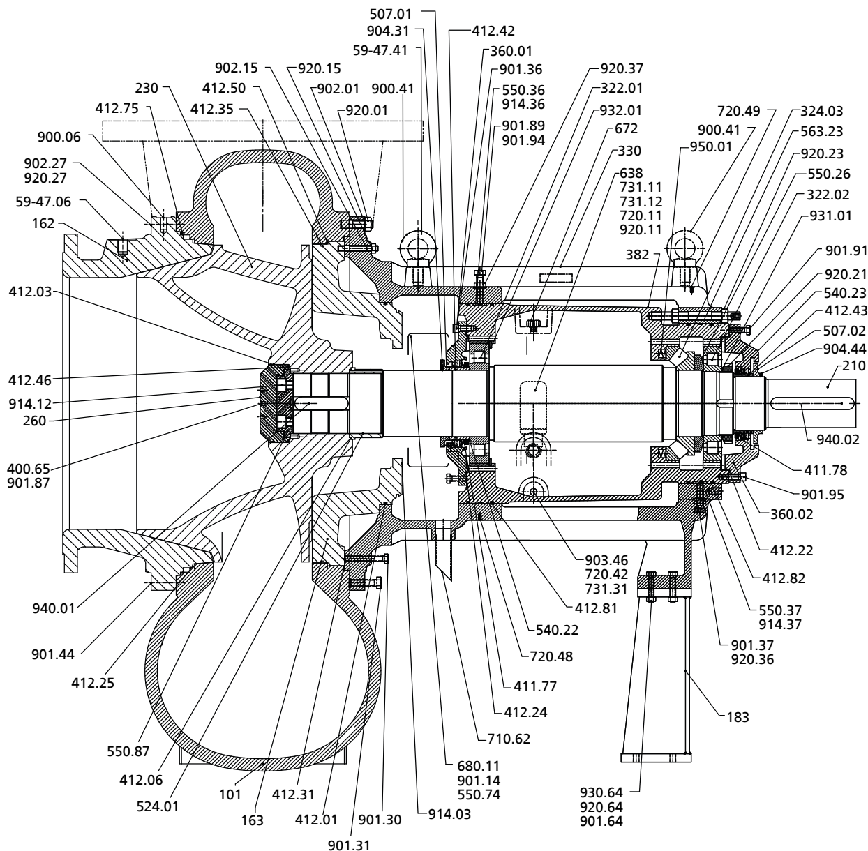
Fig. 17: General assembly drawing of pump with bearing bracket P20sx V10
