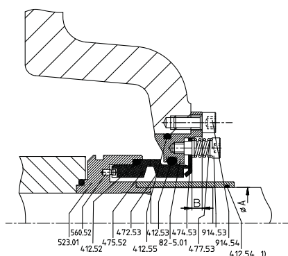
Fig. 20: 4K-120M mechanical seal 28)
