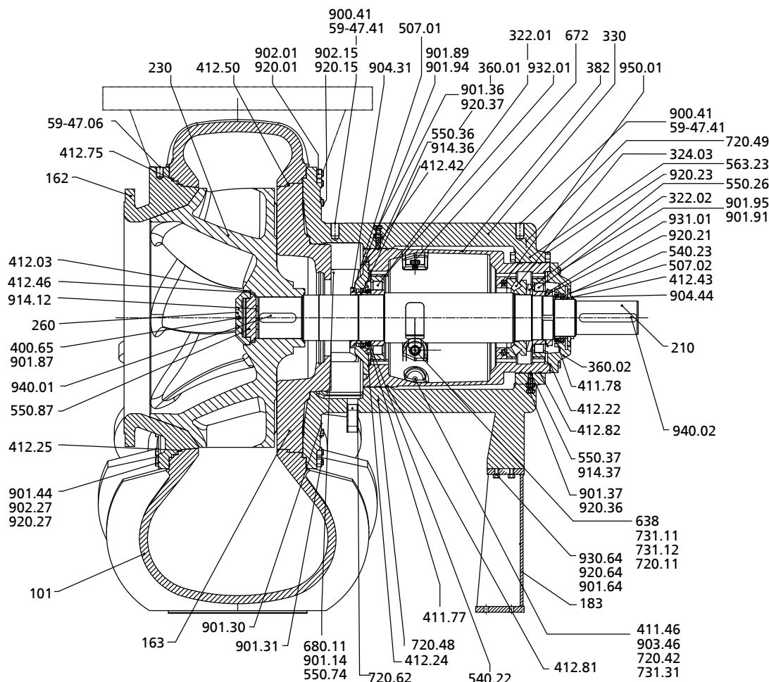
Fig. 18: General assembly drawing of pump with bearing bracket P20sx V11
