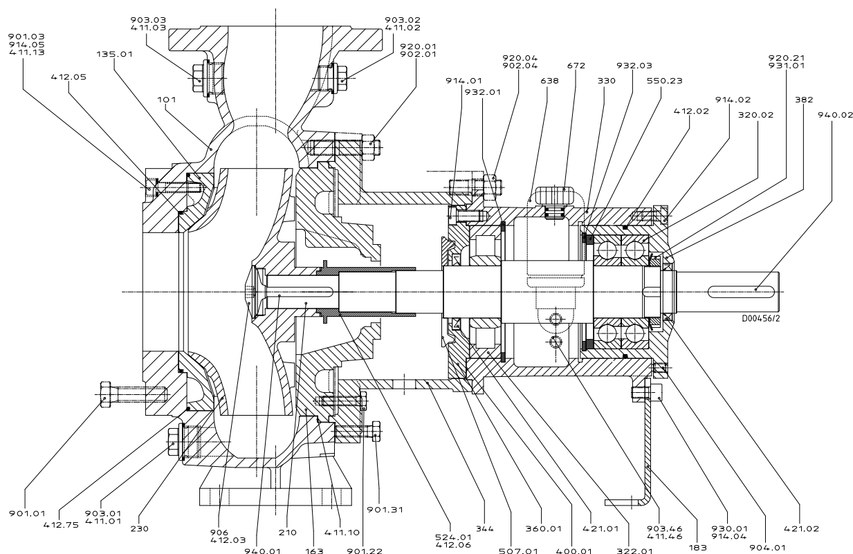
Fig. 11: General assembly drawing of pump with bearing bracket P03ax to P06x
