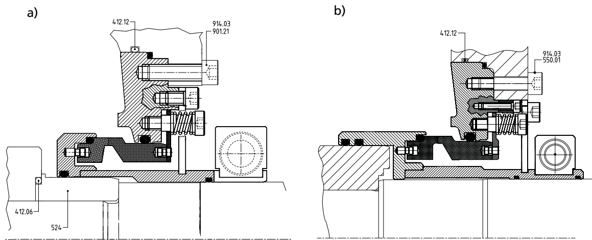
Fig. 21: Mechanical seal: a) P16ax / P20sx: 4K-160/-200 mechanical seal (for V10) b) P20sx: 4K-253 mechanical seal (for V11)
