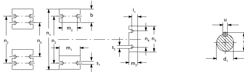
Fig. 8: Dimensions of shaft end and pump feet for pumps with bearing brackets P08sx to P12sx
