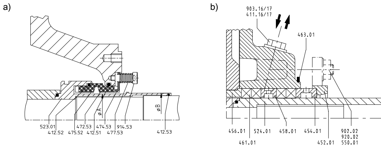
Fig. 19: Shaft seal P03ax to P12sx: a) 4K mechanical seal; b) coolable stuffing box
