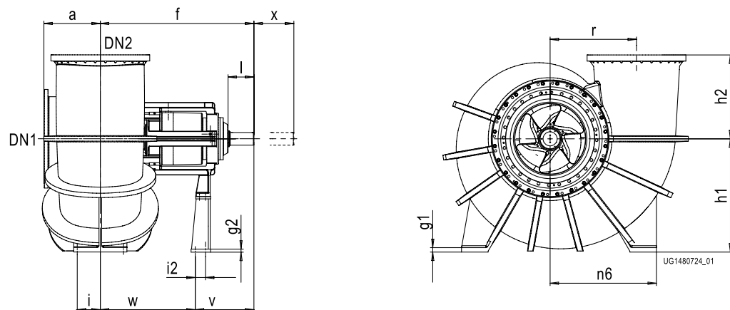
Fig. 9: Dimensions of pumps with bearing brackets P16sx and P20sx
