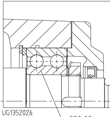
Version with bearing bracket CS40
