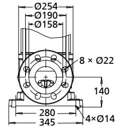
Fig. 63: Connections of Movitec VCF (PN 25, PN 40)
