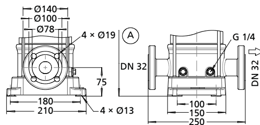
Fig. 20: Connections of Movitec VCF
