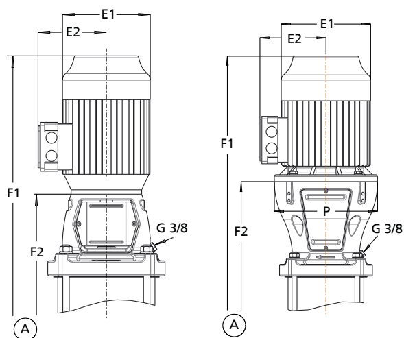
Dimensions of Movitec V(C/S)F
