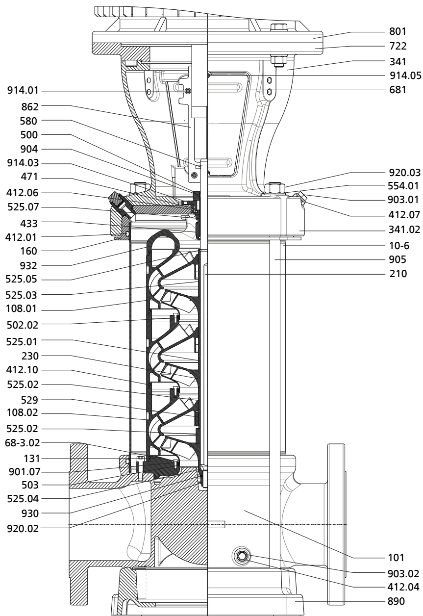
Fig. 82: General assembly drawing Movitec125B
