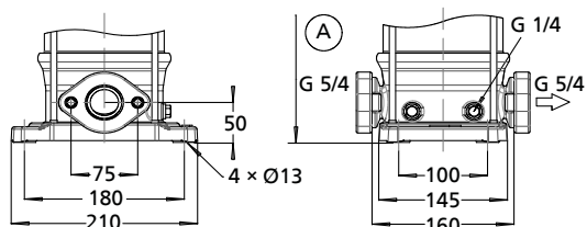
Fig. 16: Connections of Movitec V, VS
