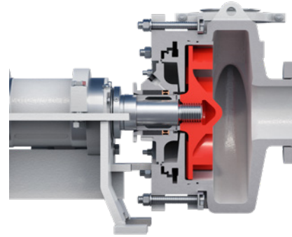
Fully recessed induced flow (Vortex) impeller:
