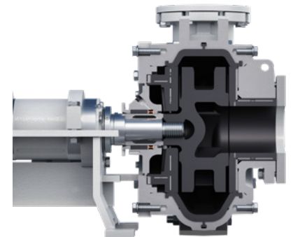
Standard closed impeller, HR pump:
