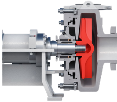
Induced flow (Vortex) impeller:
