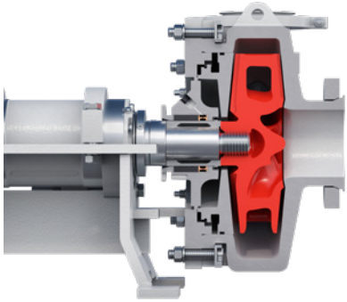
Standard closed impeller, HM pump:
