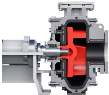
Open 3-vane impeller, HR pump:
